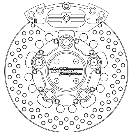
MW full floater assembly with cover plate. Cover plate has a blue anodized background and a silver foreground.
